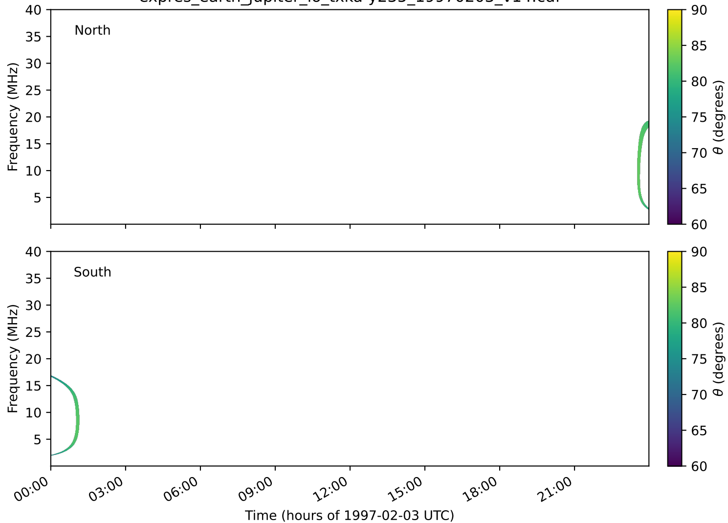
expres_earth_jupiter_io_txka-y235_19970203_v14.cdf
