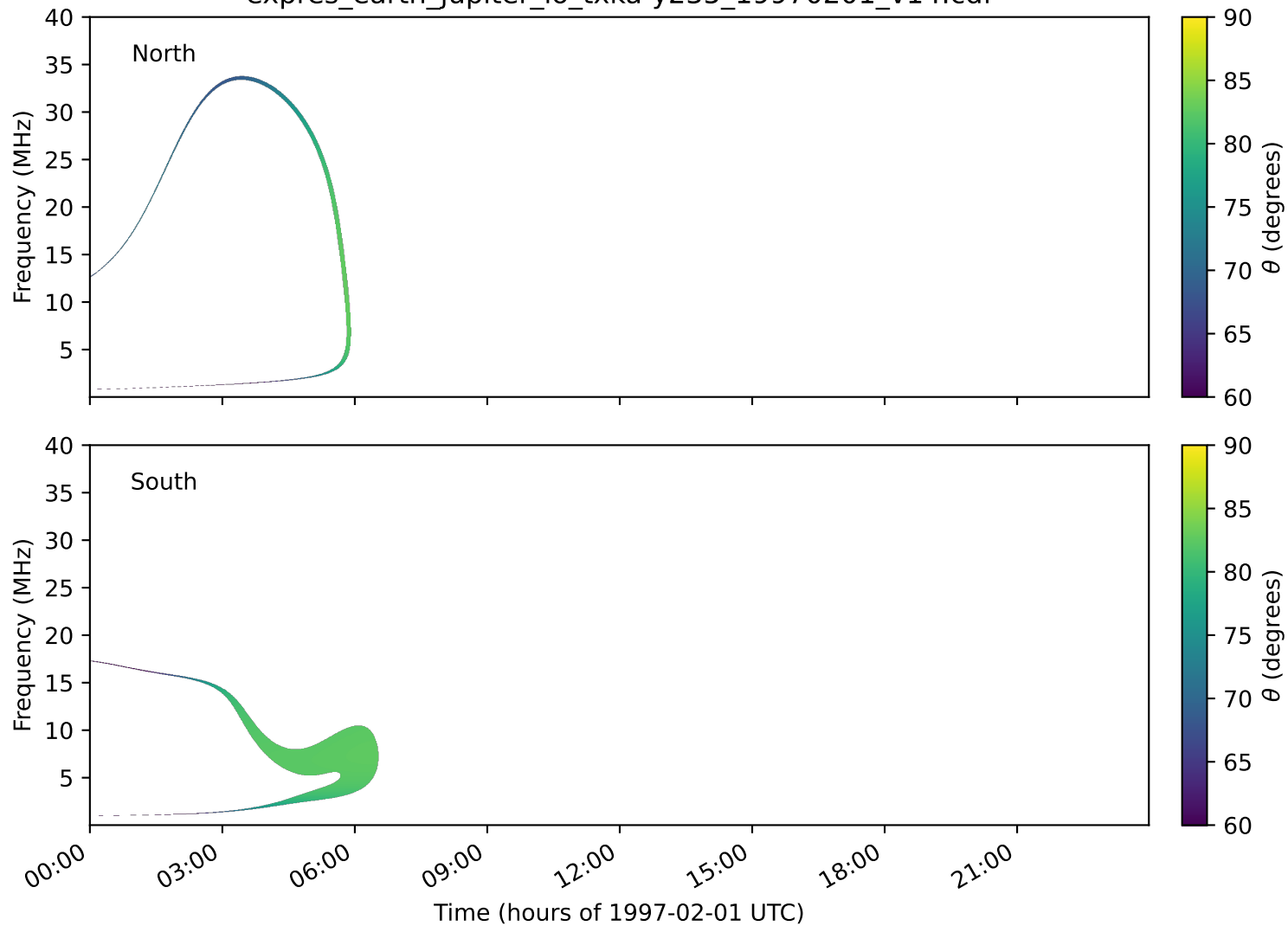
expres_earth_jupiter_io_txka-y235_19970201_v14.cdf
