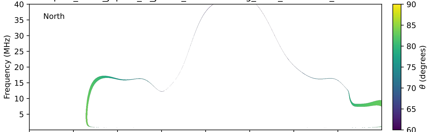
expres_earth_jupiter_io_jrm33_lossc-wid1deg_3kev_19970227_v11.cdf
