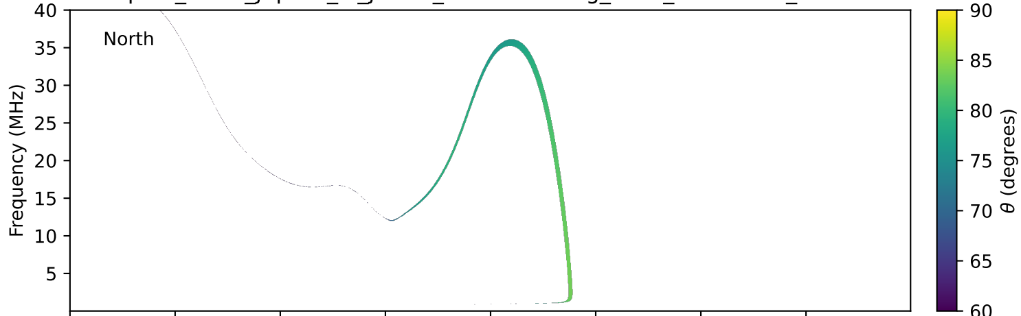
expres_earth_jupiter_io_jrm33_lossc-wid1deg_3kev_19970206_v11.cdf
