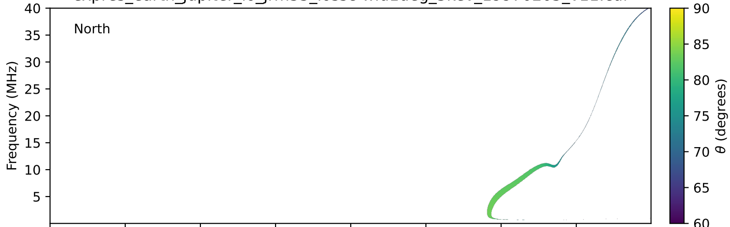
expres_earth_jupiter_io_jrm33_lossc-wid1deg_3kev_19970205_v11.cdf
