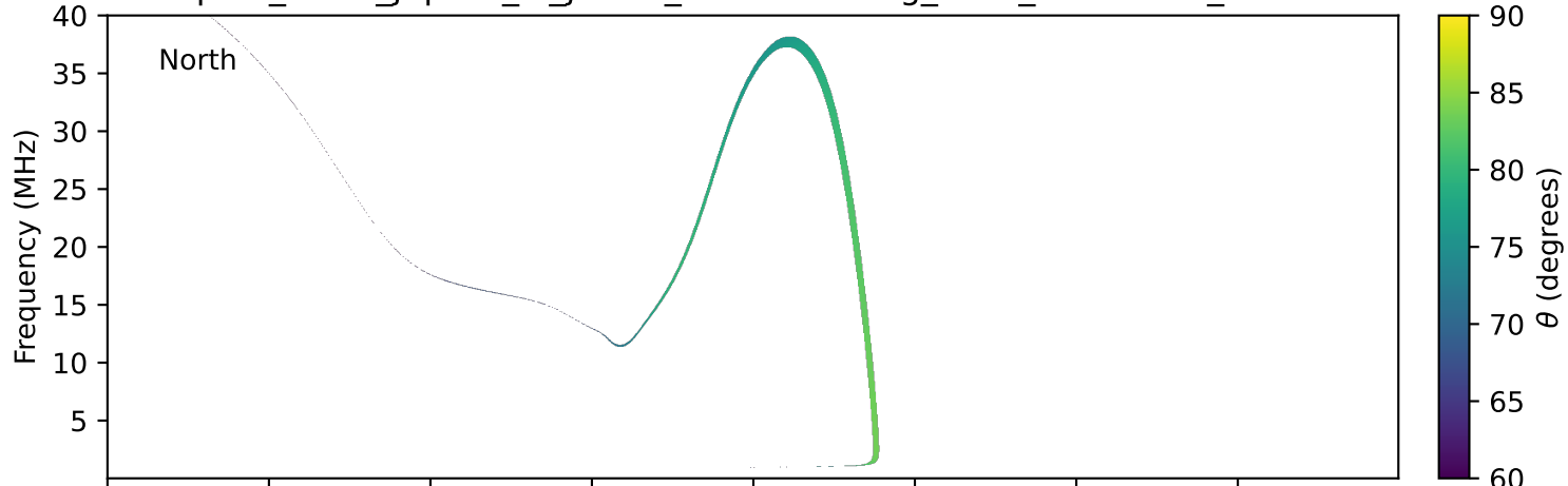
expres_earth_jupiter_io_jrm09_lossc-wid1deg_3kev_19970206_v11.cdf
