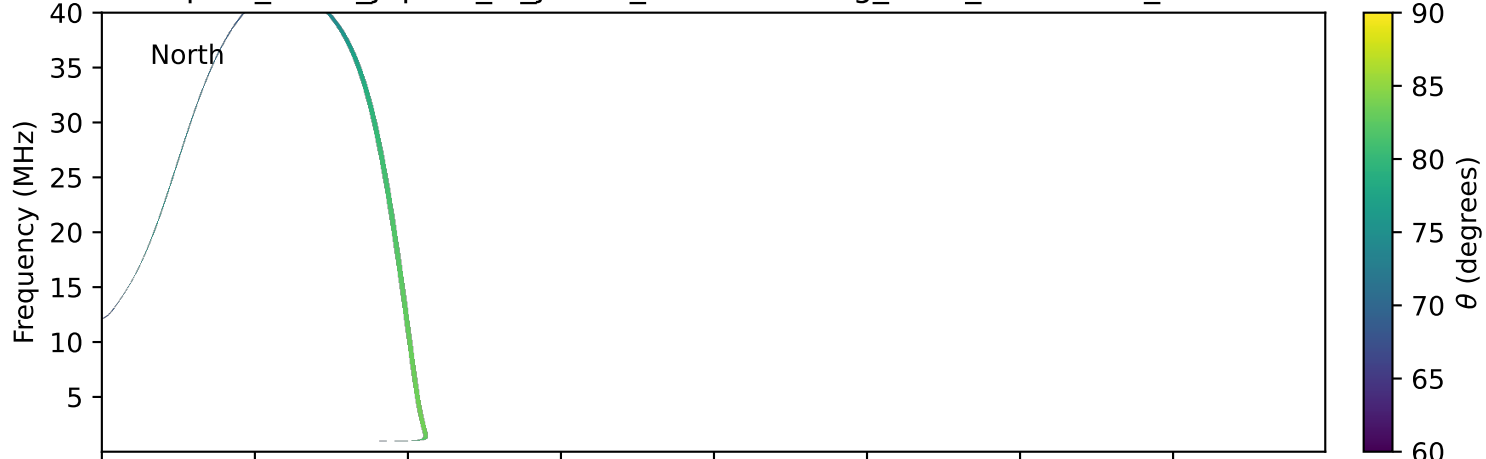
expres_earth_jupiter_io_jrm09_lossc-wid1deg_3kev_19970201_v11.cdf
