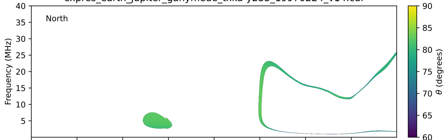
expres_earth_jupiter_ganymede_txka-y235_19970224_v14.cdf
