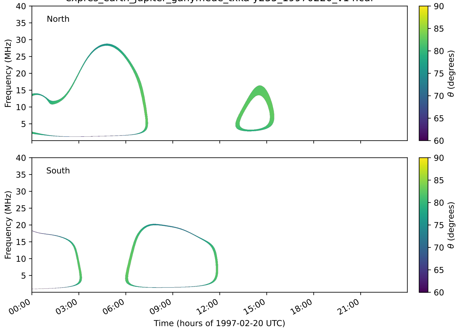
expres_earth_jupiter_ganymede_txka-y235_19970220_v14.cdf
