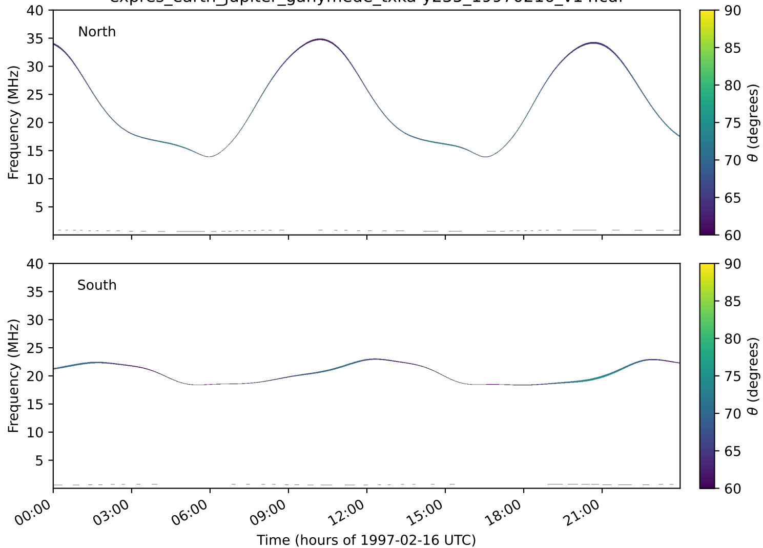
expres_earth_jupiter_ganymede_txka-y235_19970216_v14.cdf
