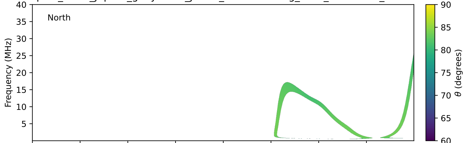
expres_earth_jupiter_ganymede_jrm33_lossc-wid1deg_3kev_19970224_v11.cdf
