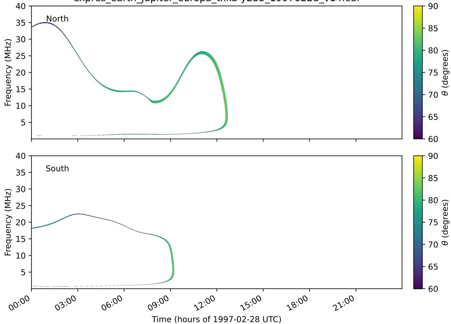
expres_earth_jupiter_europa_txka-y235_19970228_v14.cdf
