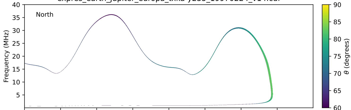
expres_earth_jupiter_europa_txka-y235_19970224_v14.cdf
