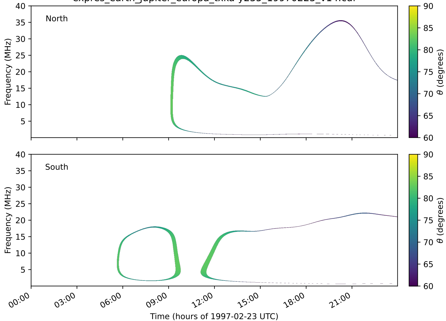
expres_earth_jupiter_europa_txka-y235_19970223_v14.cdf
