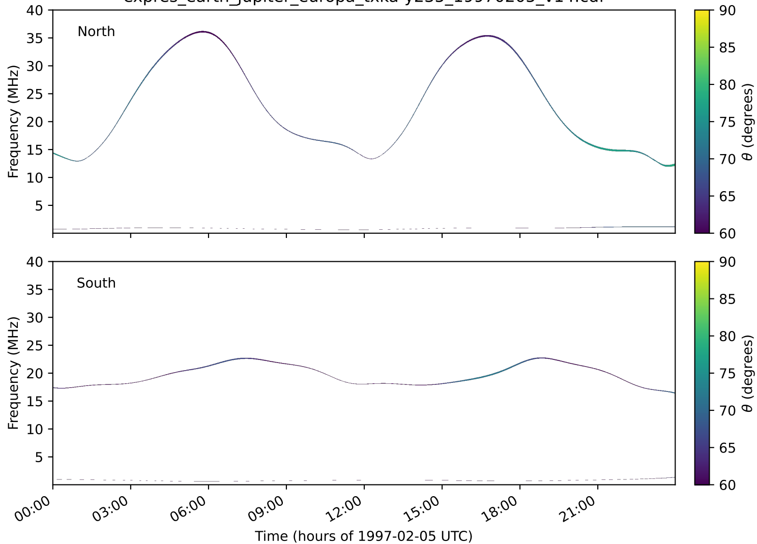
expres_earth_jupiter_europa_txka-y235_19970205_v14.cdf
