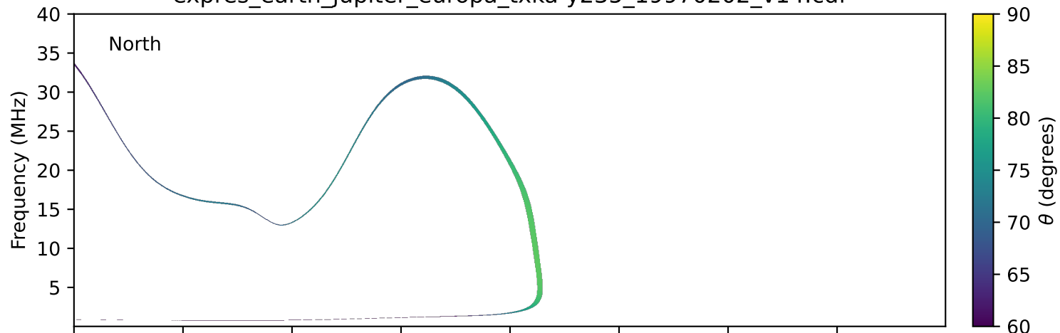
expres_earth_jupiter_europa_txka-y235_19970202_v14.cdf
