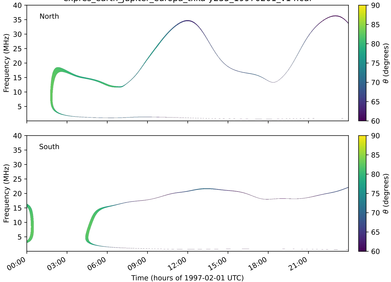
expres_earth_jupiter_europa_txka-y235_19970201_v14.cdf
