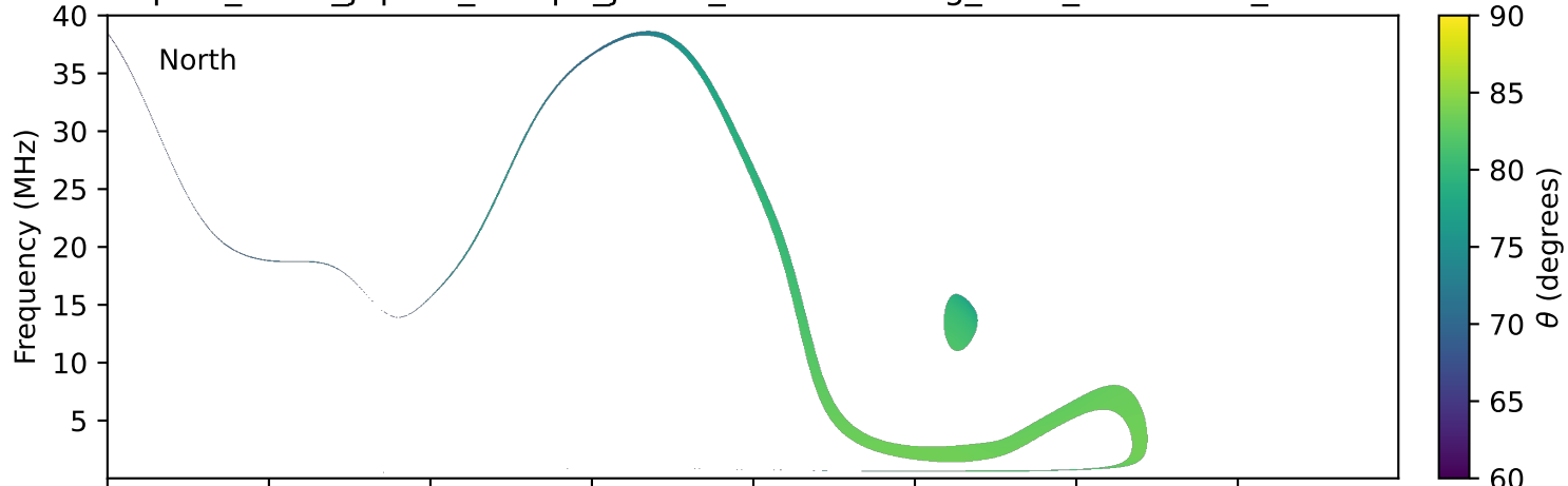
expres_earth_jupiter_europa_jrm33_lossc-wid1deg_3kev_19970202_v11.cdf
