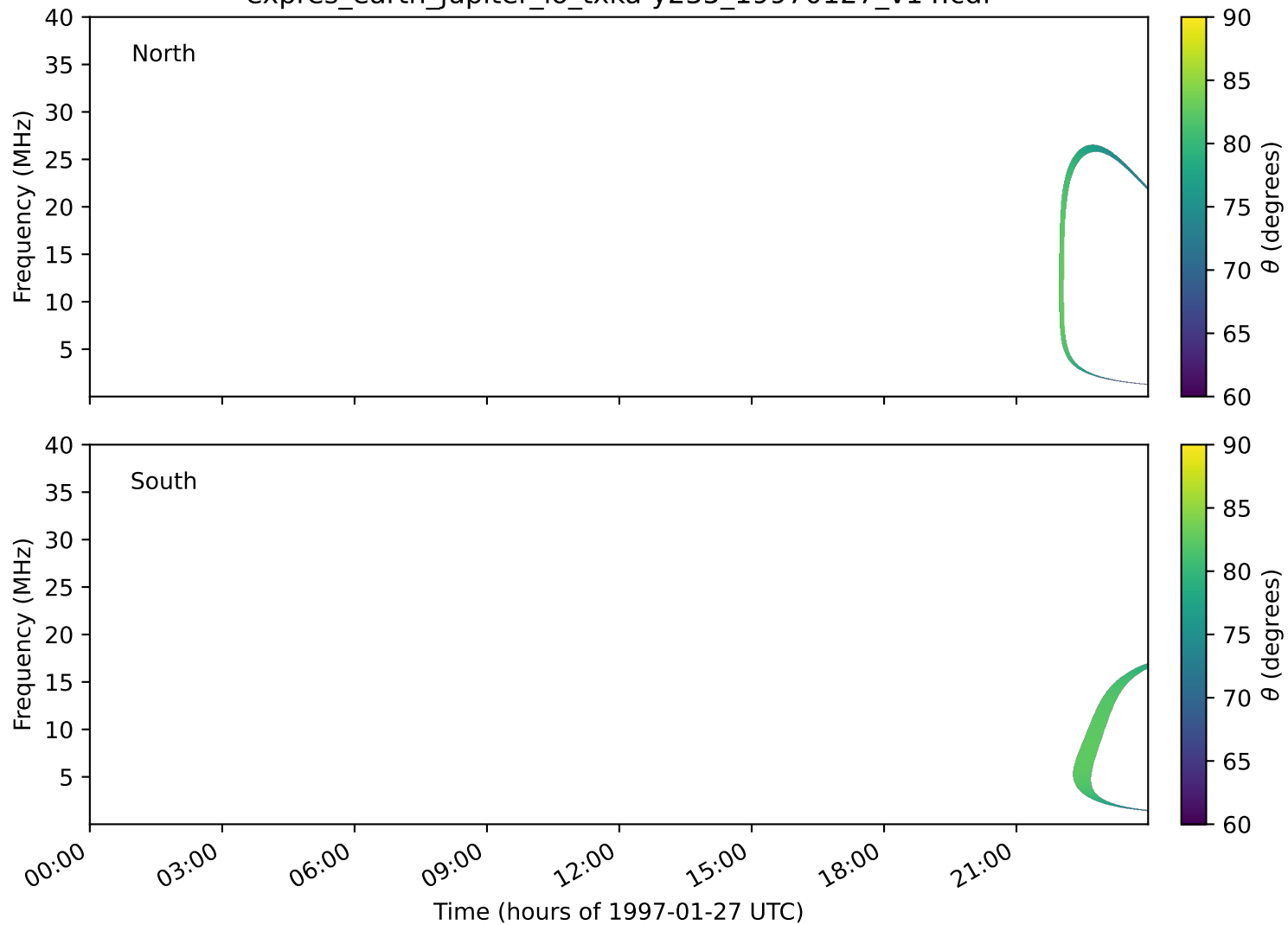
expres_earth_jupiter_io_txka-y235_19970127_v14.cdf
