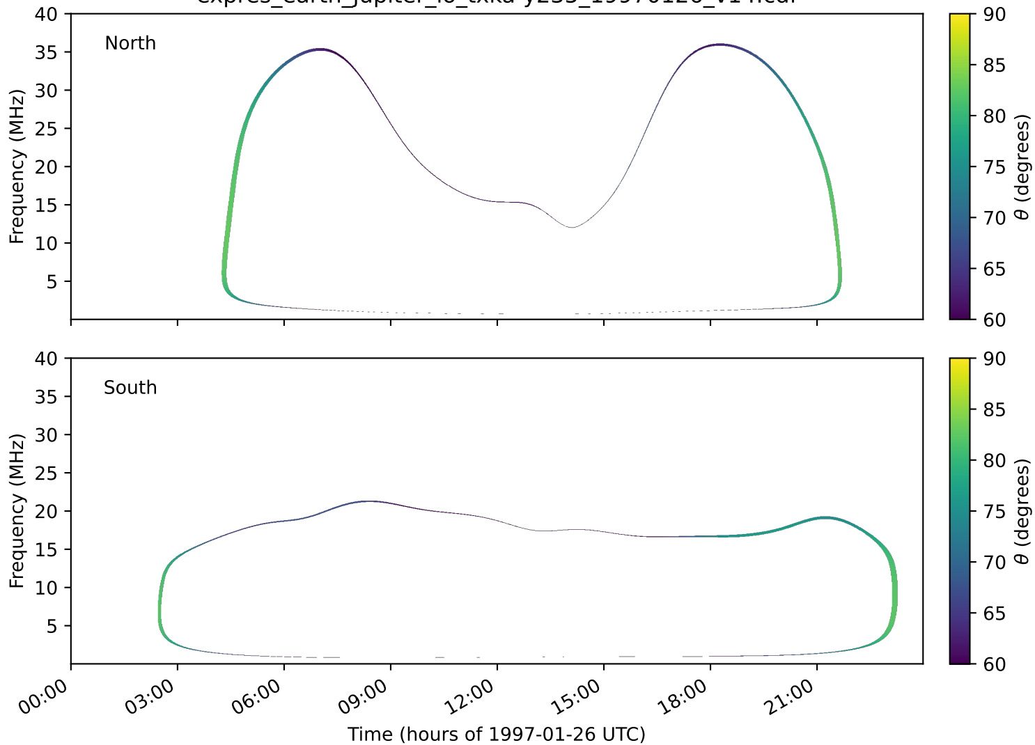
expres_earth_jupiter_io_txka-y235_19970126_v14.cdf
