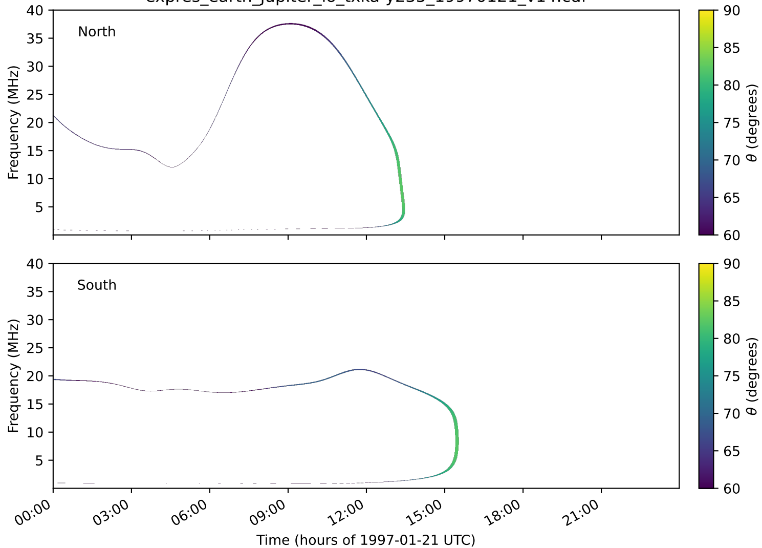
expres_earth_jupiter_io_txka-y235_19970121_v14.cdf
