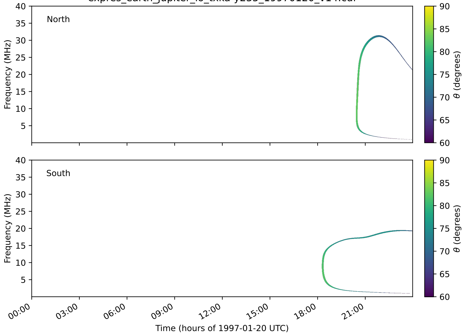
expres_earth_jupiter_io_txka-y235_19970120_v14.cdf
