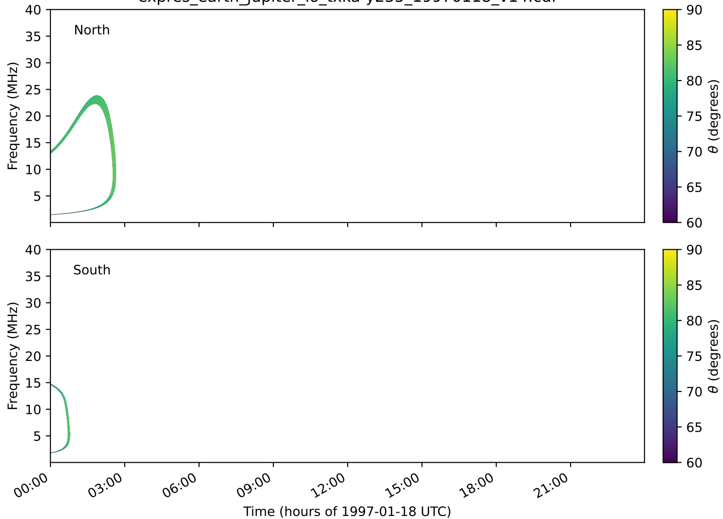
expres_earth_jupiter_io_txka-y235_19970118_v14.cdf
