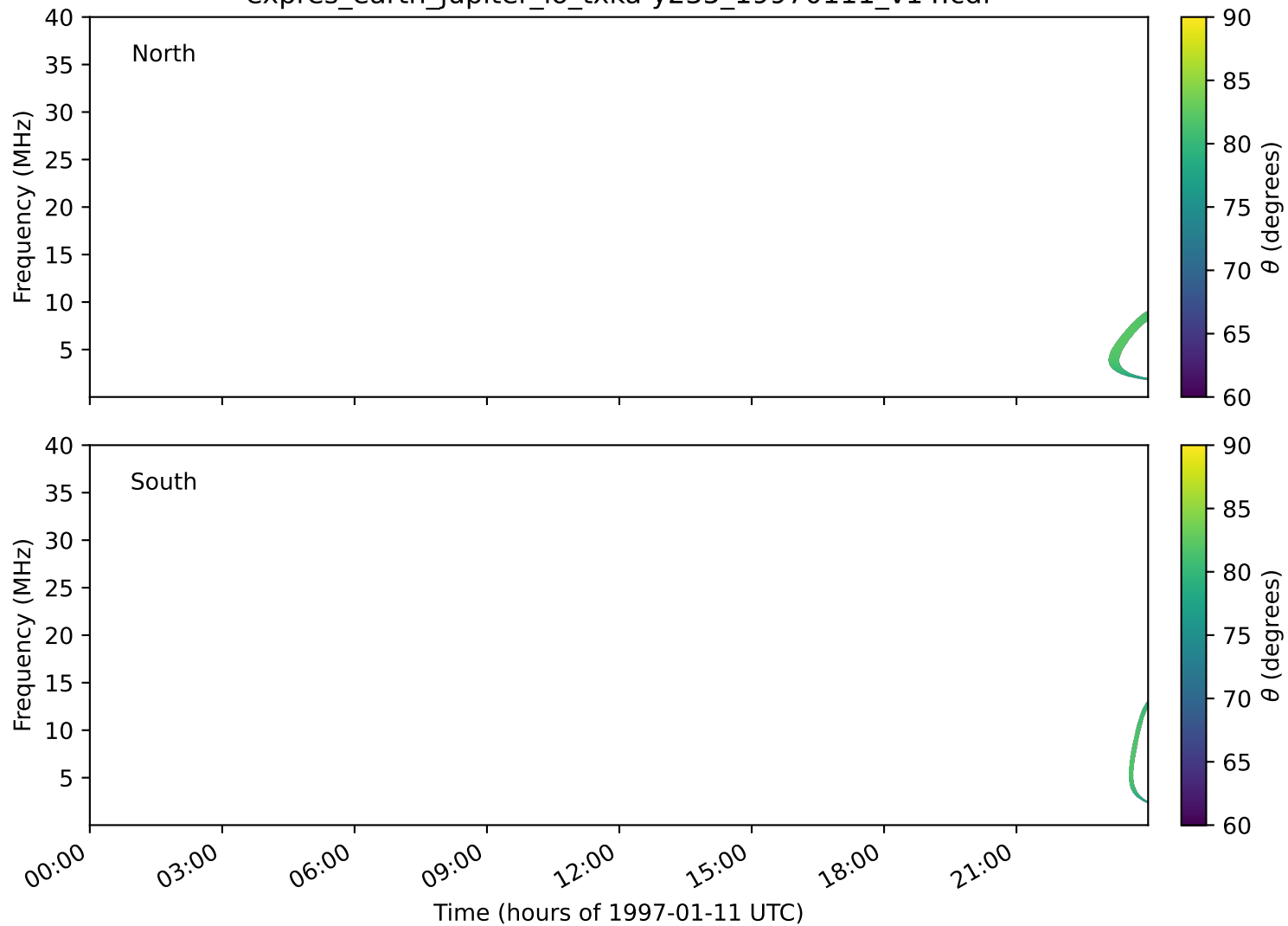
expres_earth_jupiter_io_txka-y235_19970111_v14.cdf
