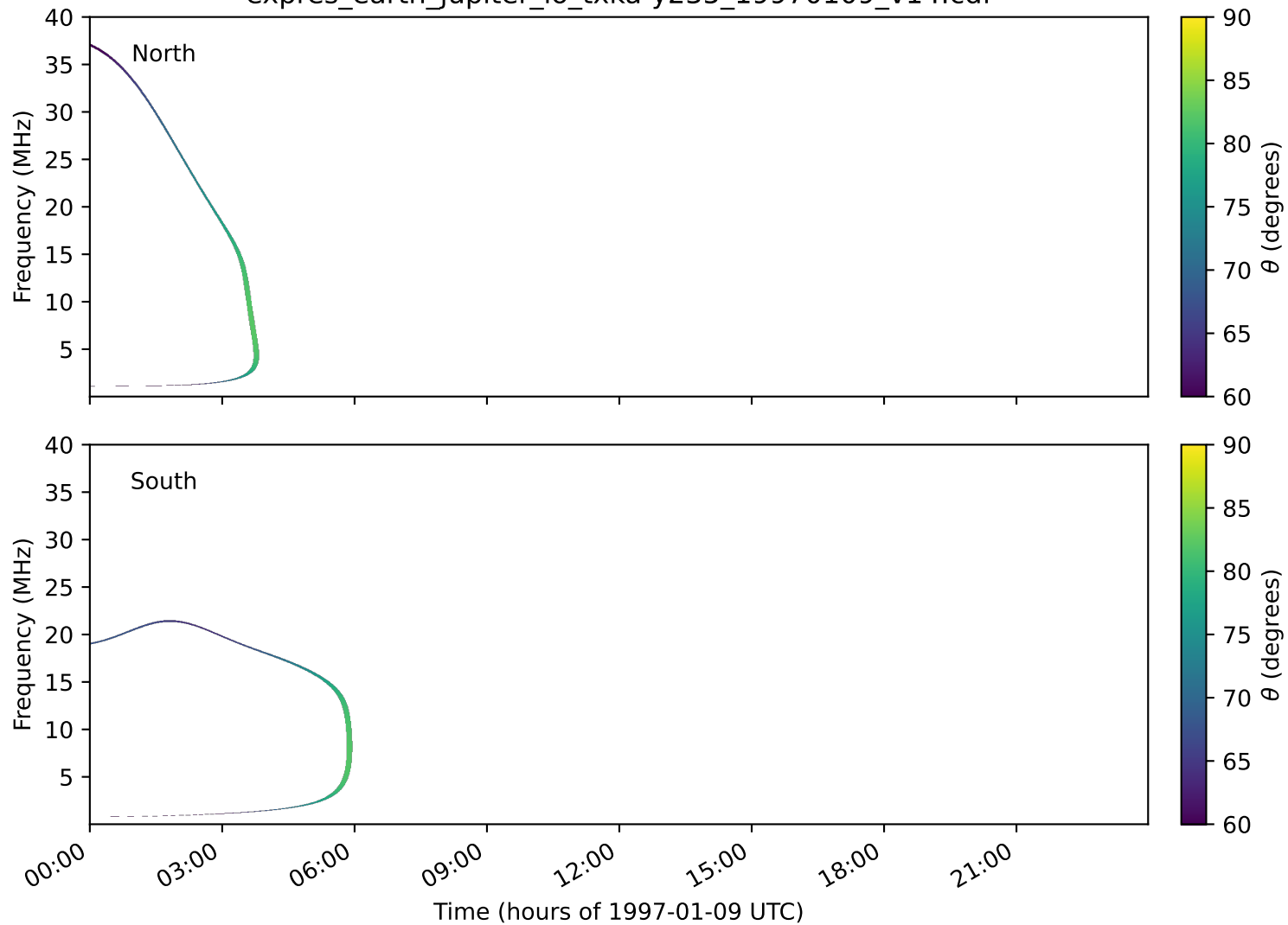
expres_earth_jupiter_io_txka-y235_19970109_v14.cdf
