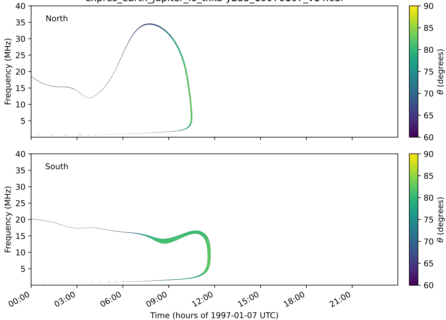
expres_earth_jupiter_io_txka-y235_19970107_v14.cdf
