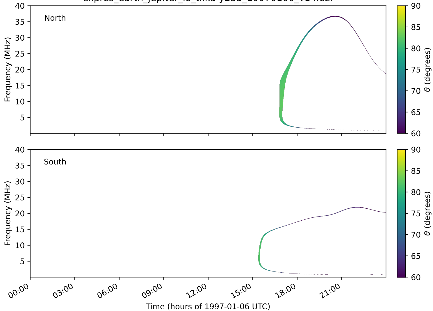
expres_earth_jupiter_io_txka-y235_19970106_v14.cdf
