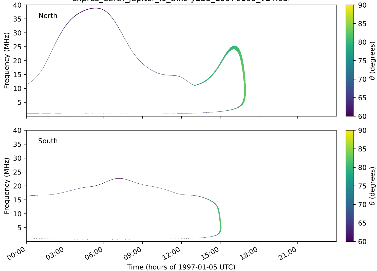
expres_earth_jupiter_io_txka-y235_19970105_v14.cdf
