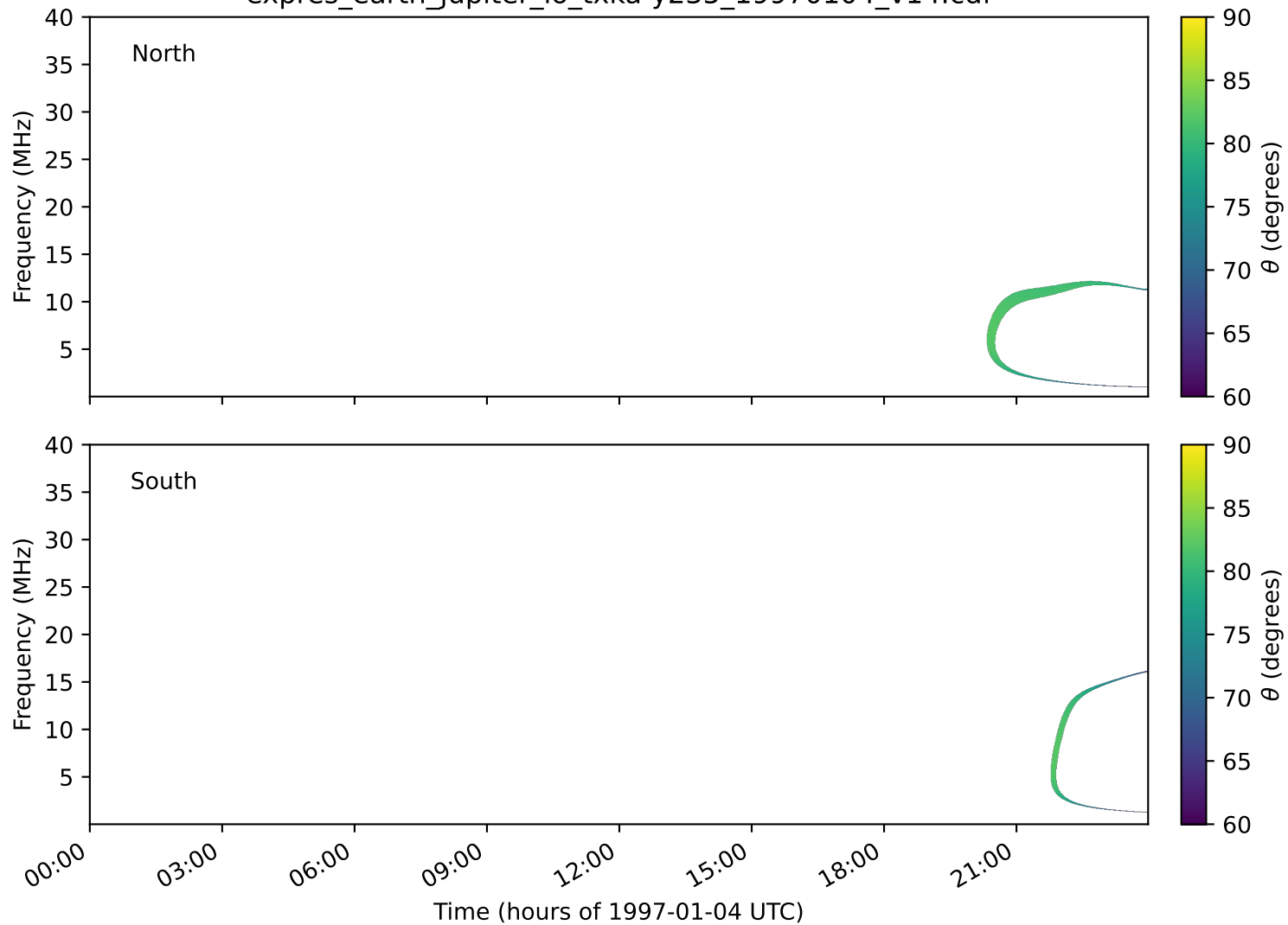
expres_earth_jupiter_io_txka-y235_19970104_v14.cdf
