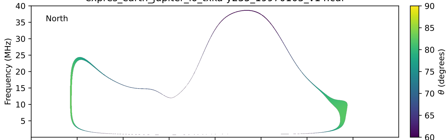
expres_earth_jupiter_io_txka-y235_19970103_v14.cdf
