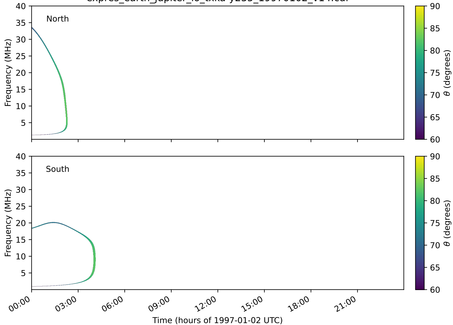
expres_earth_jupiter_io_txka-y235_19970102_v14.cdf
