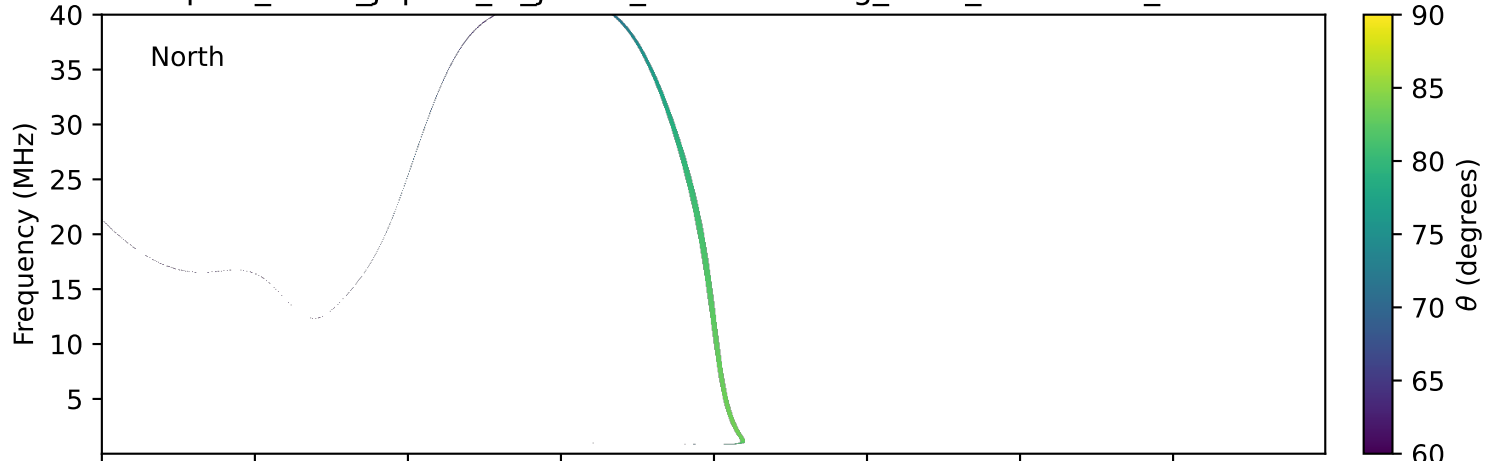
expres_earth_jupiter_io_jrm33_lossc-wid1deg_3kev_19970114_v11.cdf
