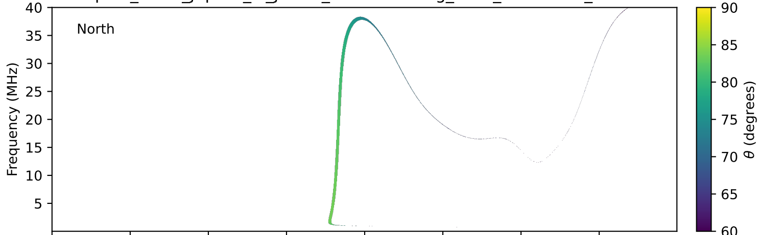
expres_earth_jupiter_io_jrm33_lossc-wid1deg_3kev_19970108_v11.cdf
