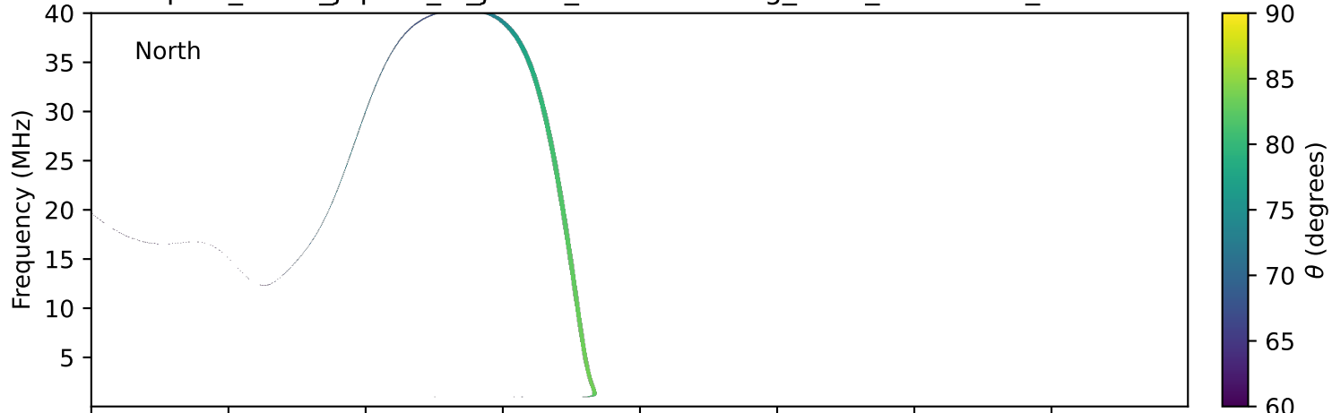
expres_earth_jupiter_io_jrm33_lossc-wid1deg_3kev_19970107_v11.cdf
