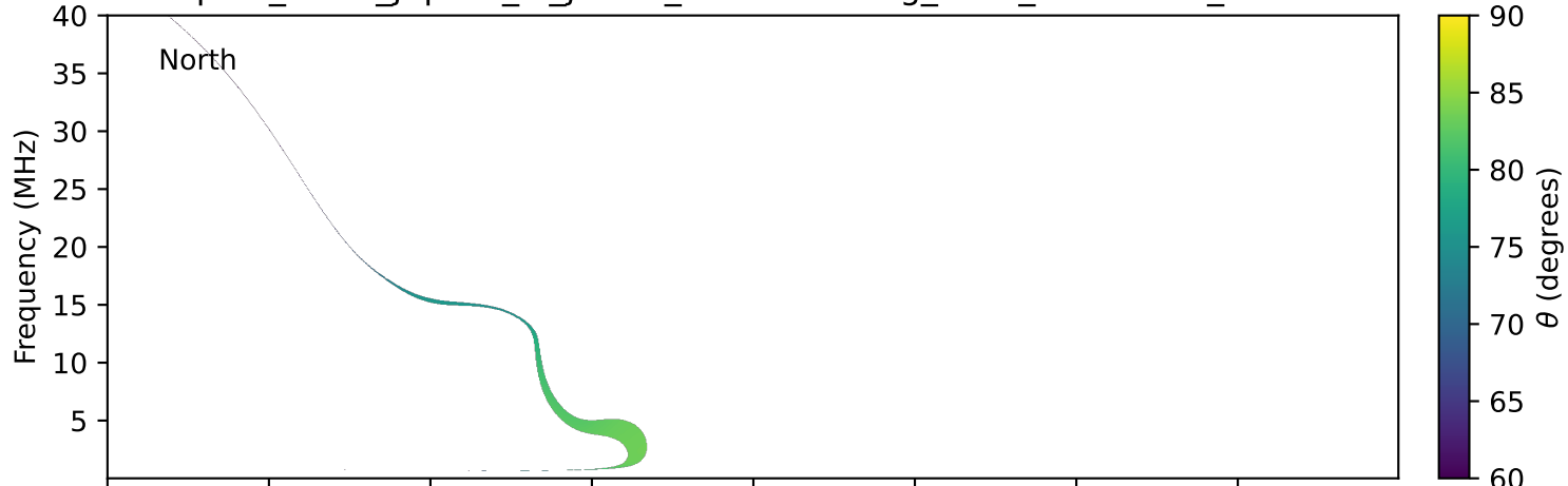
expres_earth_jupiter_io_jrm09_lossc-wid1deg_3kev_19970123_v11.cdf
