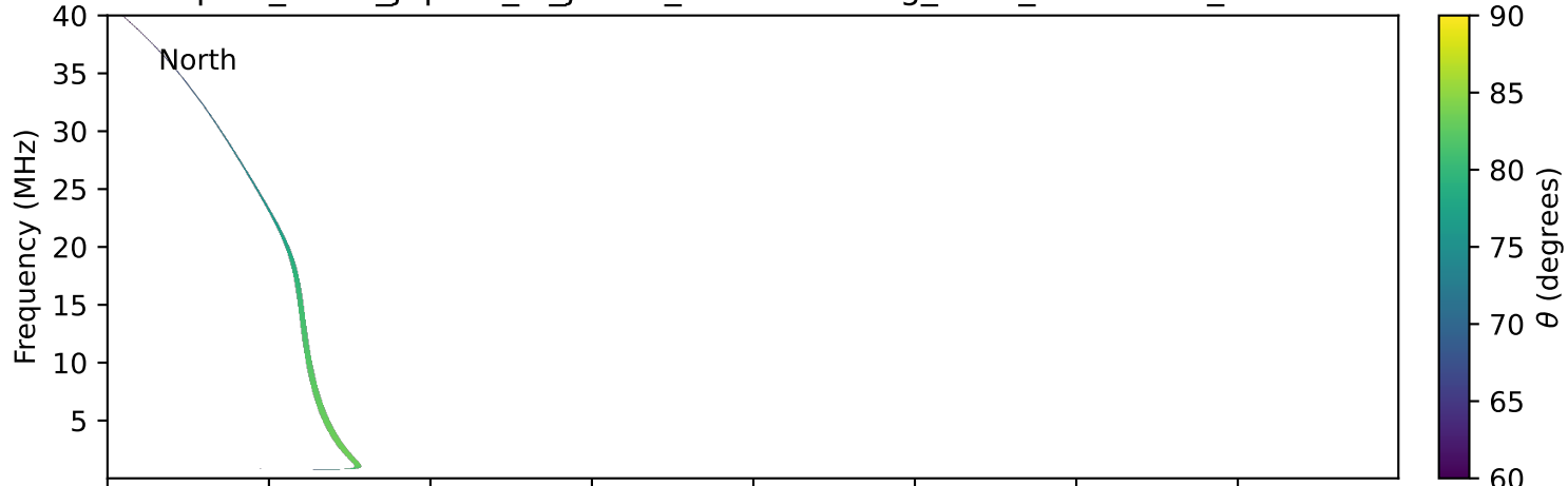
expres_earth_jupiter_io_jrm09_lossc-wid1deg_3kev_19970109_v11.cdf
