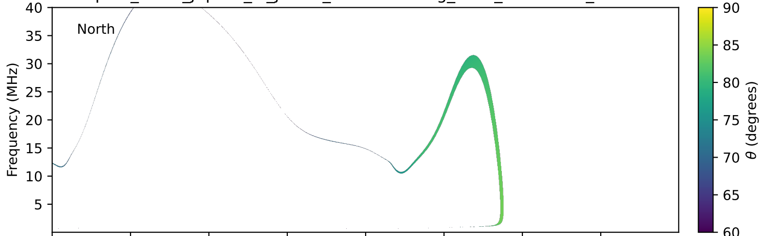
expres_earth_jupiter_io_jrm09_lossc-wid1deg_3kev_19970105_v11.cdf
