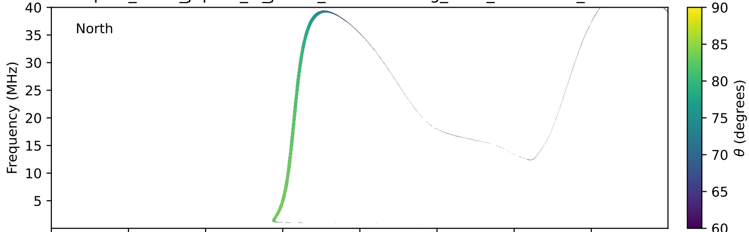
expres_earth_jupiter_io_jrm09_lossc-wid1deg_3kev_19970101_v11.cdf
