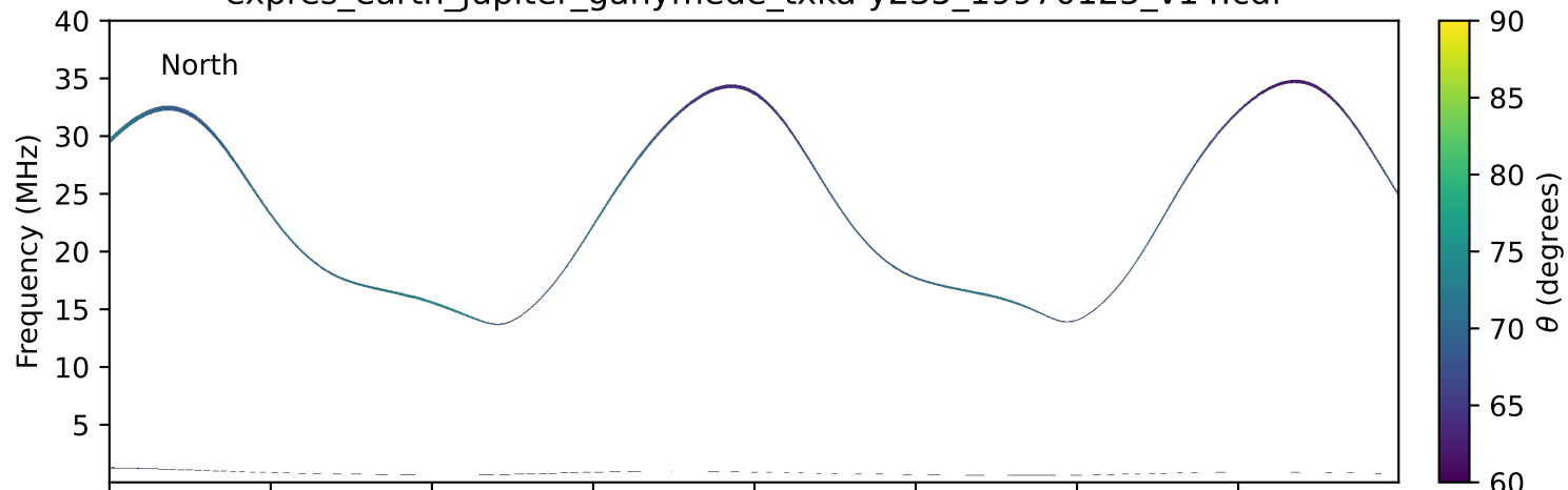
expres_earth_jupiter_ganymede_txka-y235_19970125_v14.cdf
