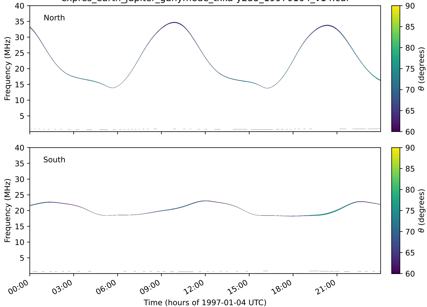
expres_earth_jupiter_ganymede_txka-y235_19970104_v14.cdf
