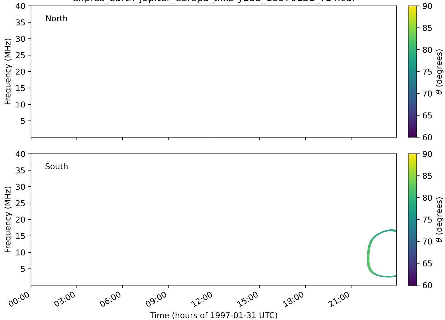
expres_earth_jupiter_europa_txka-y235_19970131_v14.cdf
