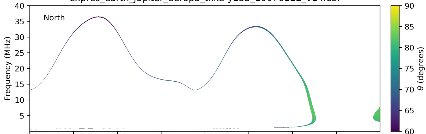
expres_earth_jupiter_europa_txka-y235_19970122_v14.cdf
