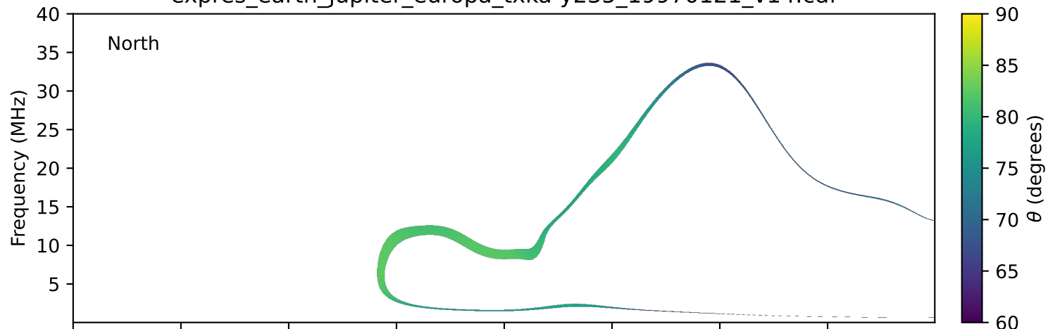
expres_earth_jupiter_europa_txka-y235_19970121_v14.cdf
