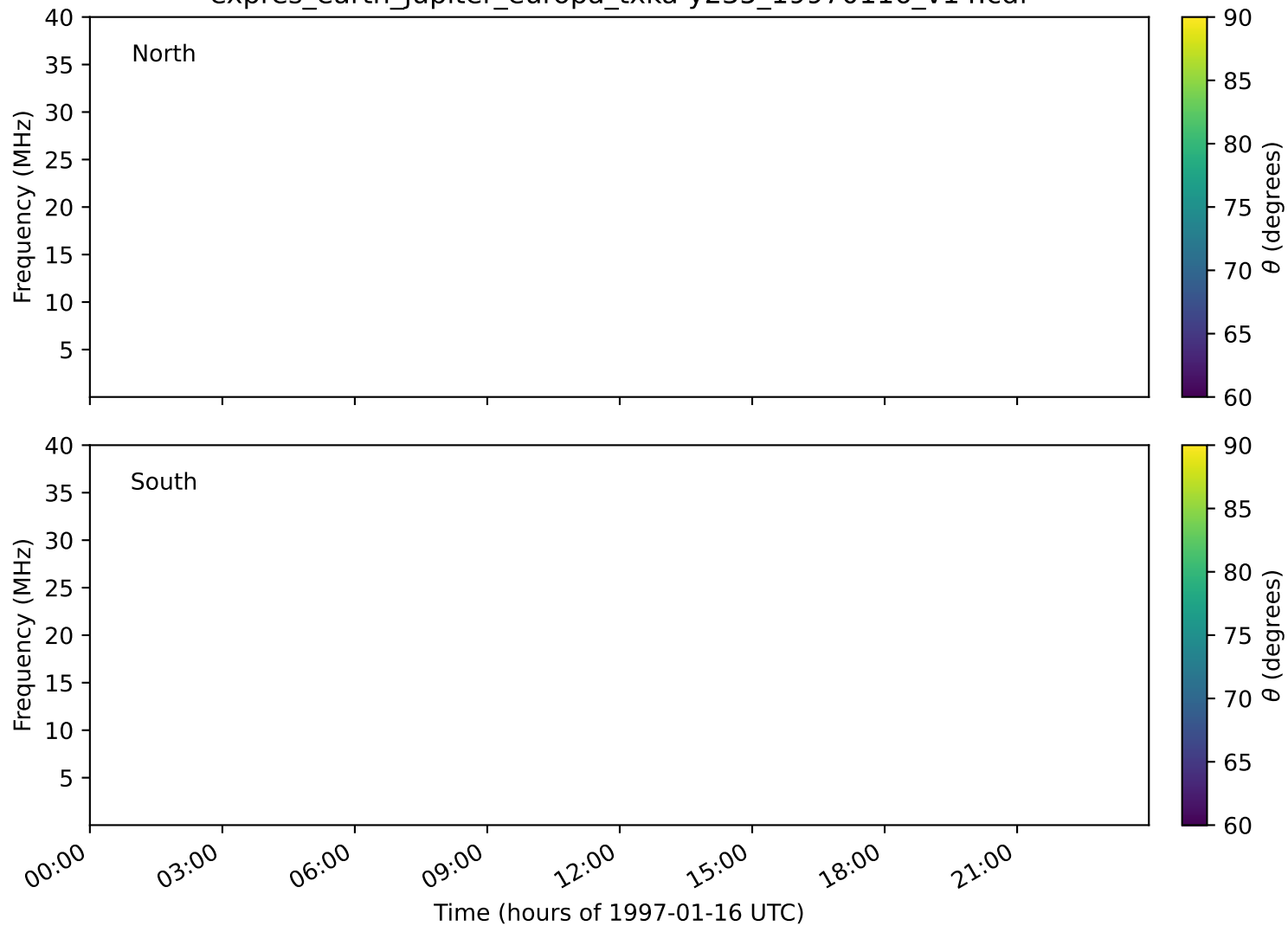
expres_earth_jupiter_europa_txka-y235_19970116_v14.cdf
