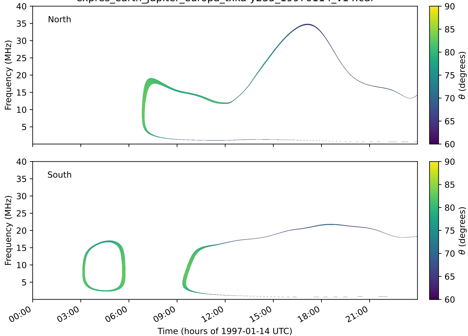
expres_earth_jupiter_europa_txka-y235_19970114_v14.cdf
