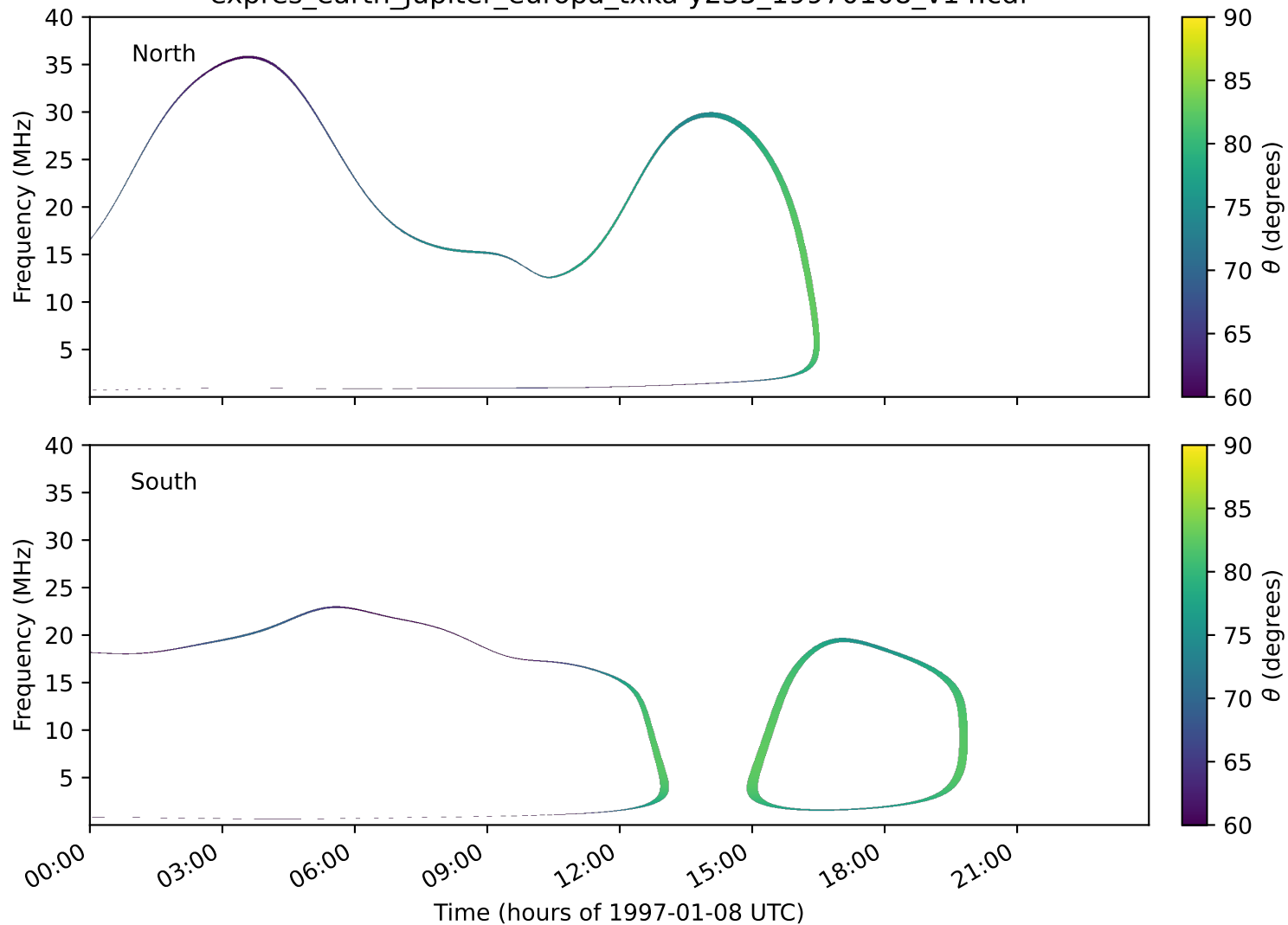
expres_earth_jupiter_europa_txka-y235_19970108_v14.cdf
