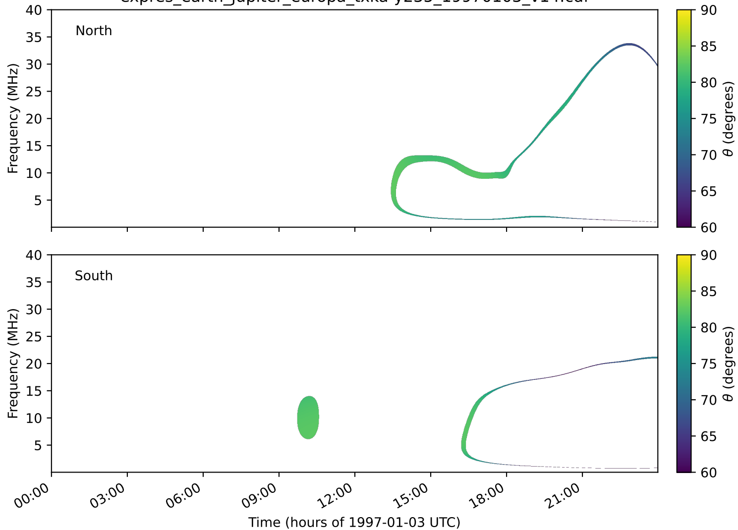
expres_earth_jupiter_europa_txka-y235_19970103_v14.cdf
