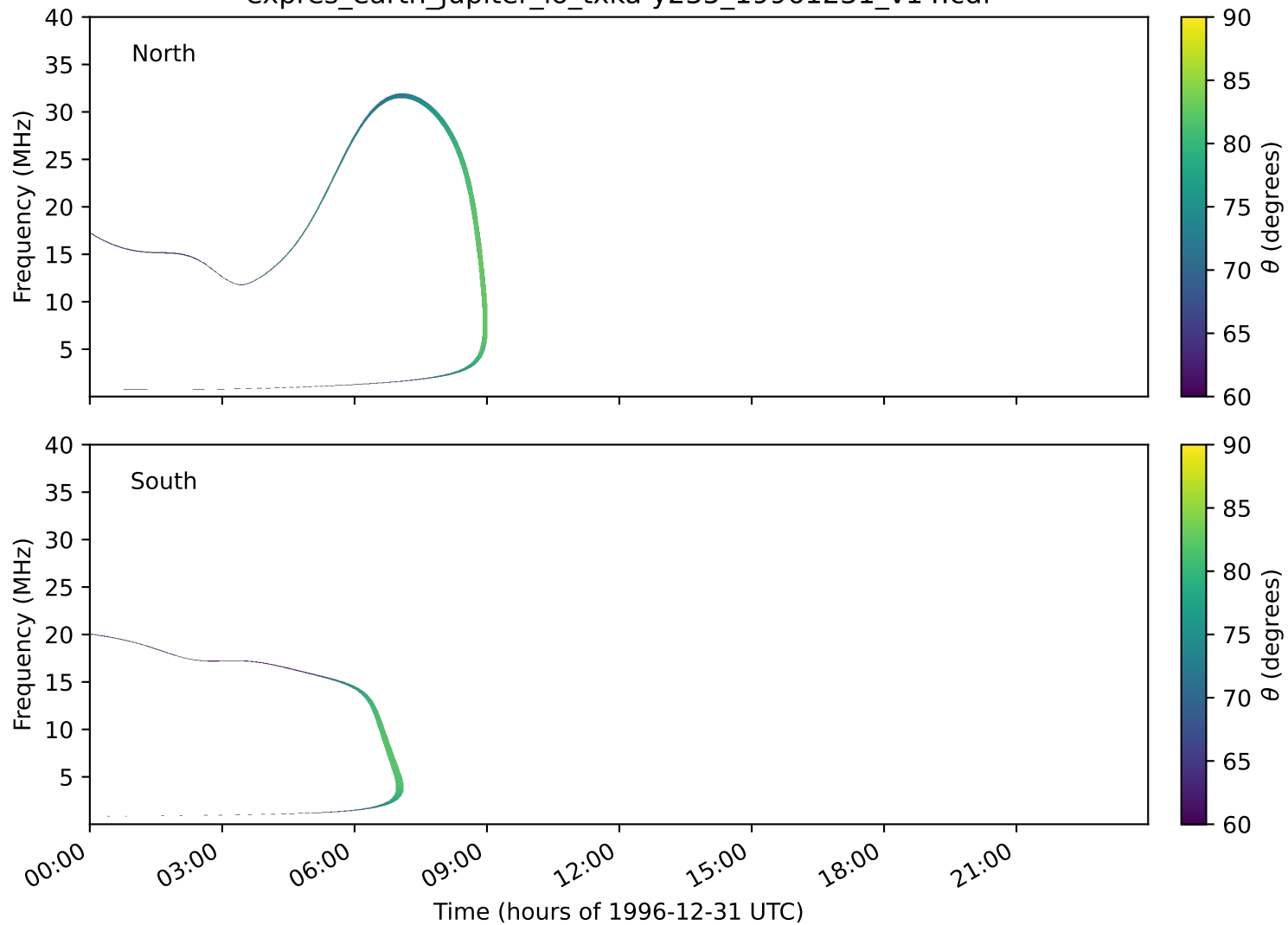
expres_earth_jupiter_io_txka-y235_19961231_v14.cdf
