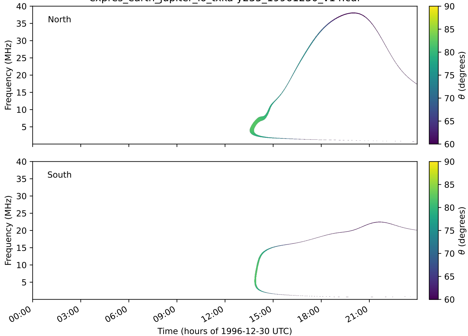
expres_earth_jupiter_io_txka-y235_19961230_v14.cdf
