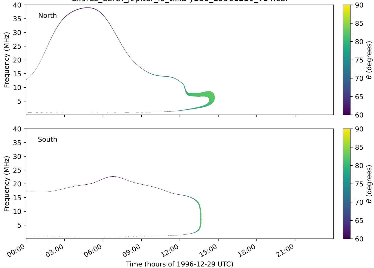
expres_earth_jupiter_io_txka-y235_19961229_v14.cdf
